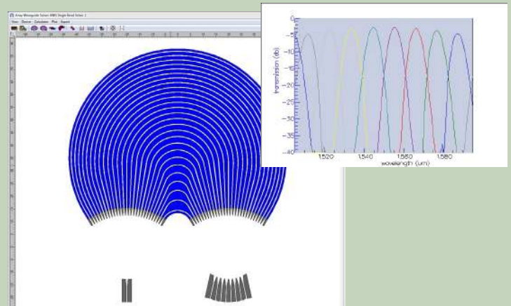
AWG: varying radius single bend
