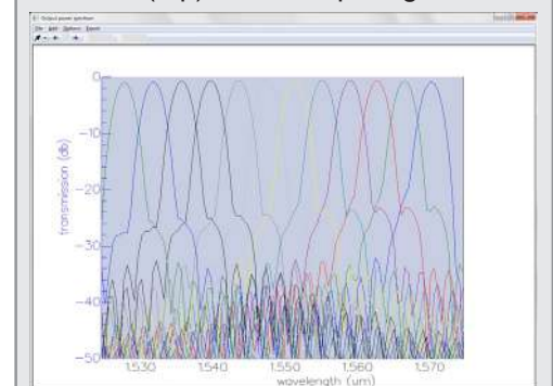
(bottom) with tapering - note the additional shoulders (cross-talk)
