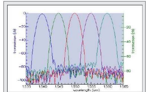
(bottom) with MMIs, (top) without
