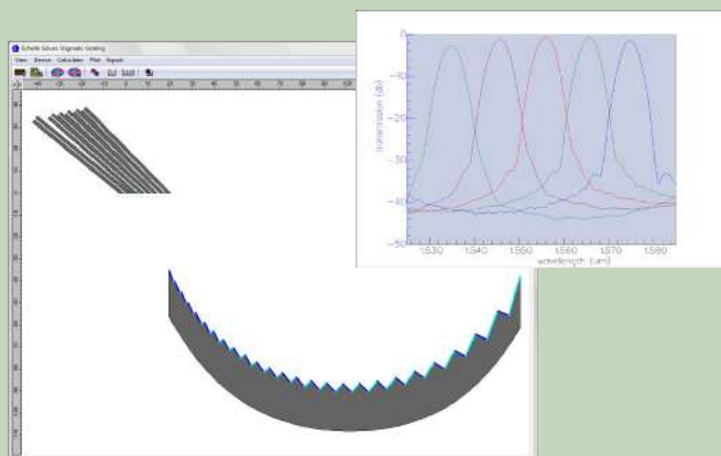
Echelle: stigmatic design
