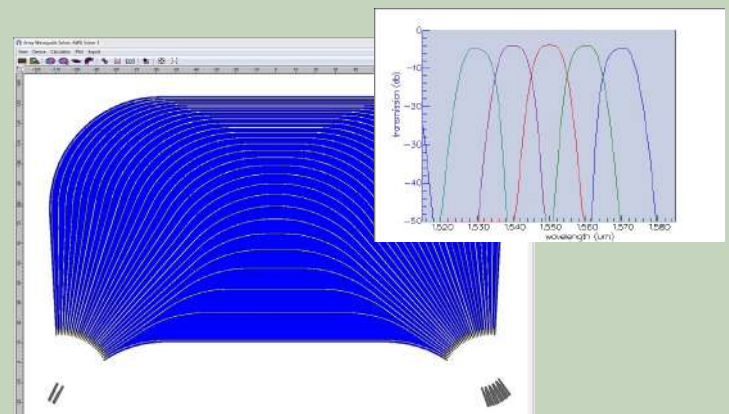
AWG: fixed radius double bend with MMIs
